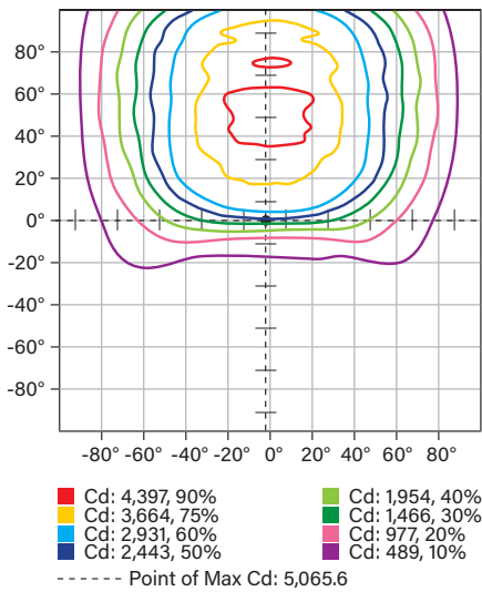
ISOCANDELA PLOT
